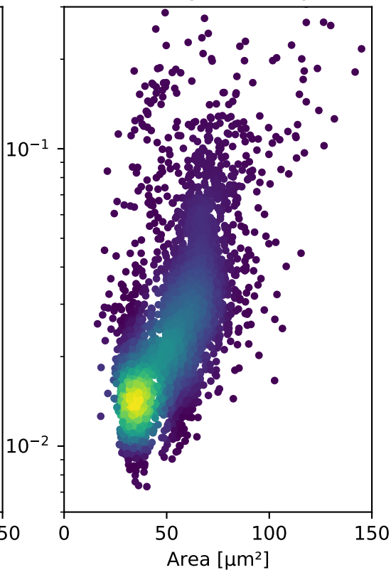
KDE with logarithmic y-scale
